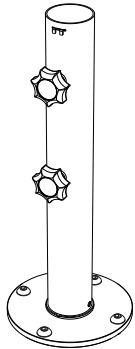
Centre Pole Tube 4 x M10 x 20 button head screws
